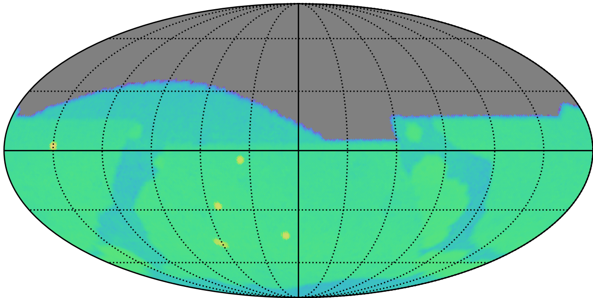
too_elab_r16_d2_giz_v3.4_10yrs g: SurfaceBrightLimit
