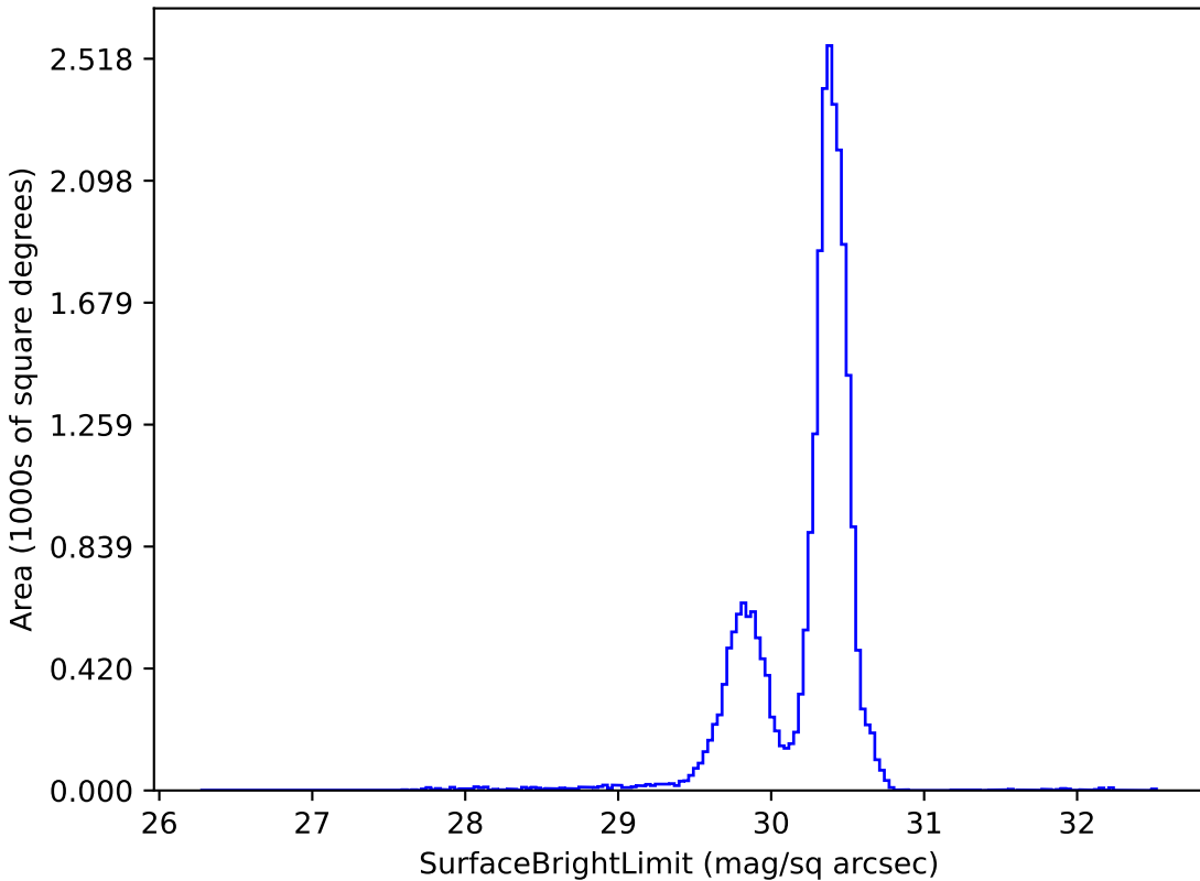
too_elab_r16_d2_giz_v3.4_10yrs g: SurfaceBrightLimit
