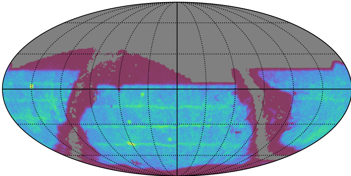
too_elab_r16_d2_giz_v3.4_10yrs : SNSLMetric
