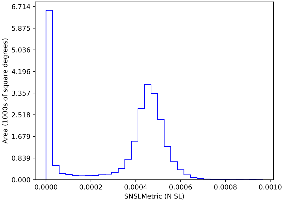
too_elab_r16_d2_giz_v3.4_10yrs : SNSLMetric
