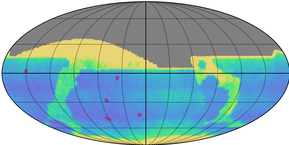
too_elab_r16_d2_giz_v3.4_10yrs : Proper Motion Uncert @ 24.0
