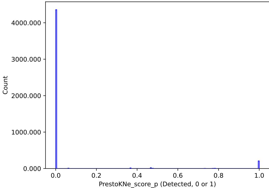
too_elab_r16_d2_giz_v3.4_10yrs : PrestoKNe_score_p
