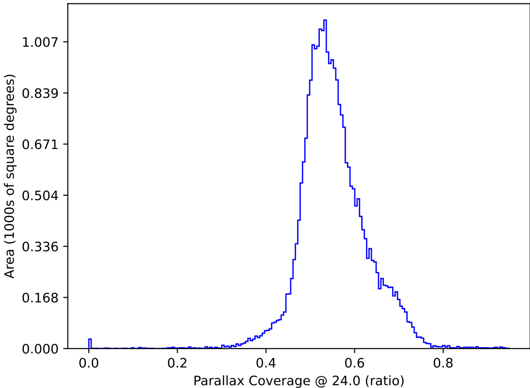
too_elab_r16_d2_giz_v3.4_10yrs : Parallax Coverage @ 24.0
