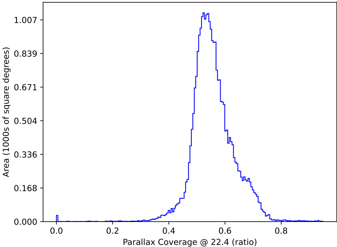
too_elab_r16_d2_giz_v3.4_10yrs : Parallax Coverage @ 22.4
