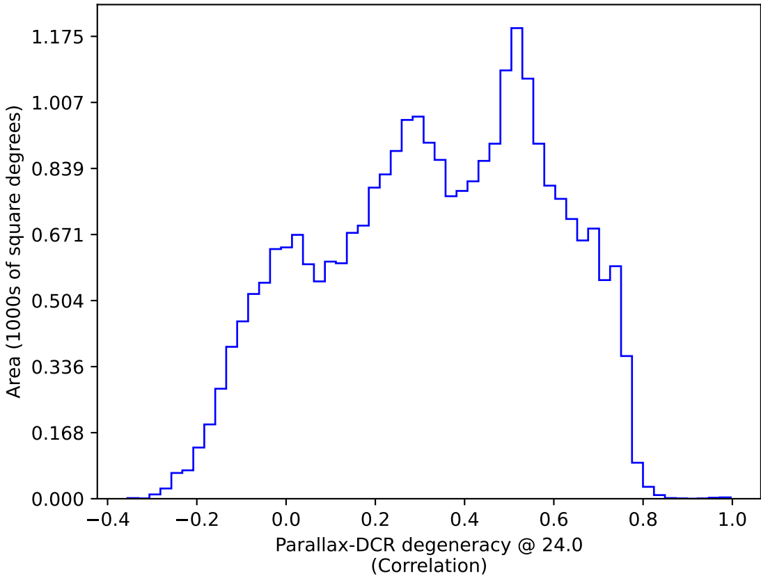
too_elab_r16_d2_giz_v3.4_10yrs : Parallax-DCR degeneracy @ 24.0
