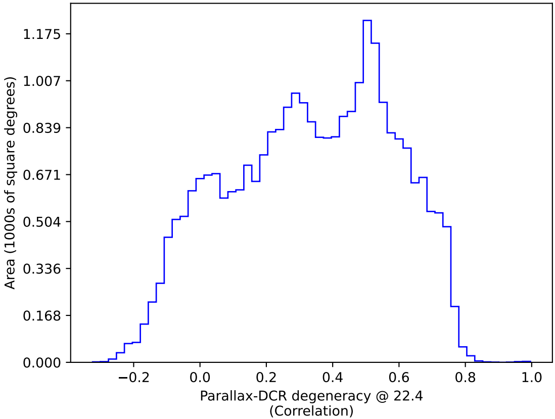
too_elab_r16_d2_giz_v3.4_10yrs : Parallax-DCR degeneracy @ 22.4
