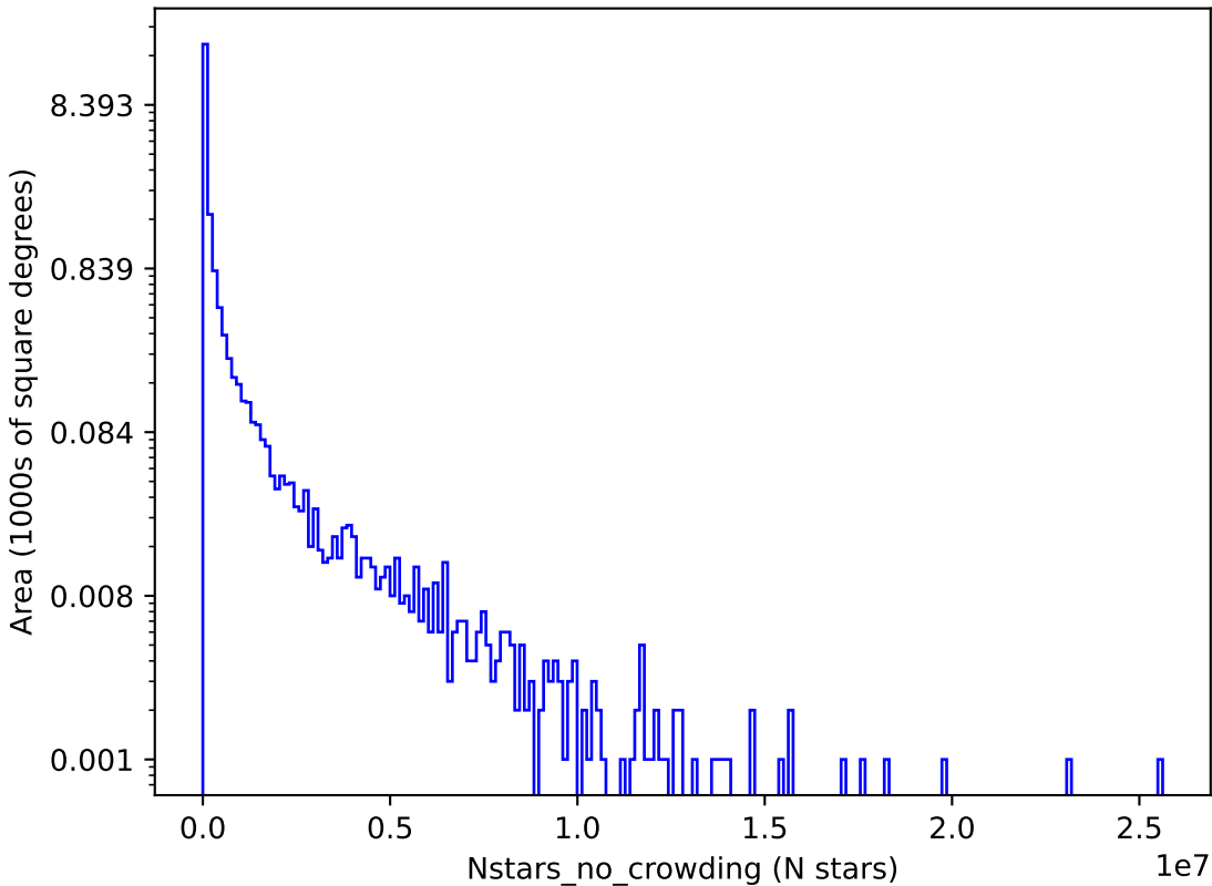
too_elab_r16_d2_giz_v3.4_10yrs y: Nstars_no_crowding
