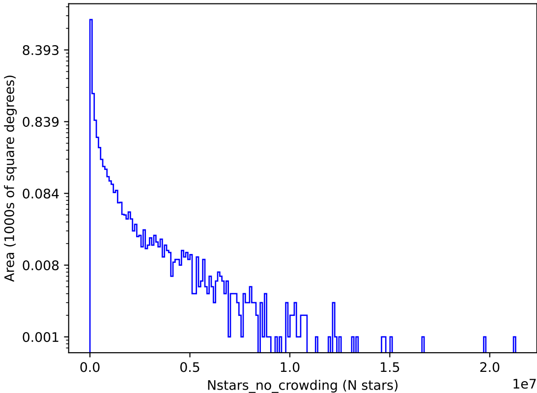
too_elab_r16_d2_giz_v3.4_10yrs r: Nstars_no_crowding
