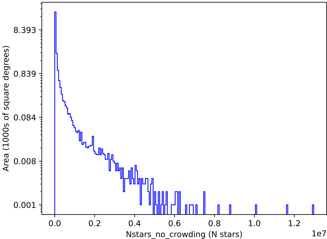
too_elab_r16_d2_giz_v3.4_10yrs g: Nstars_no_crowding
