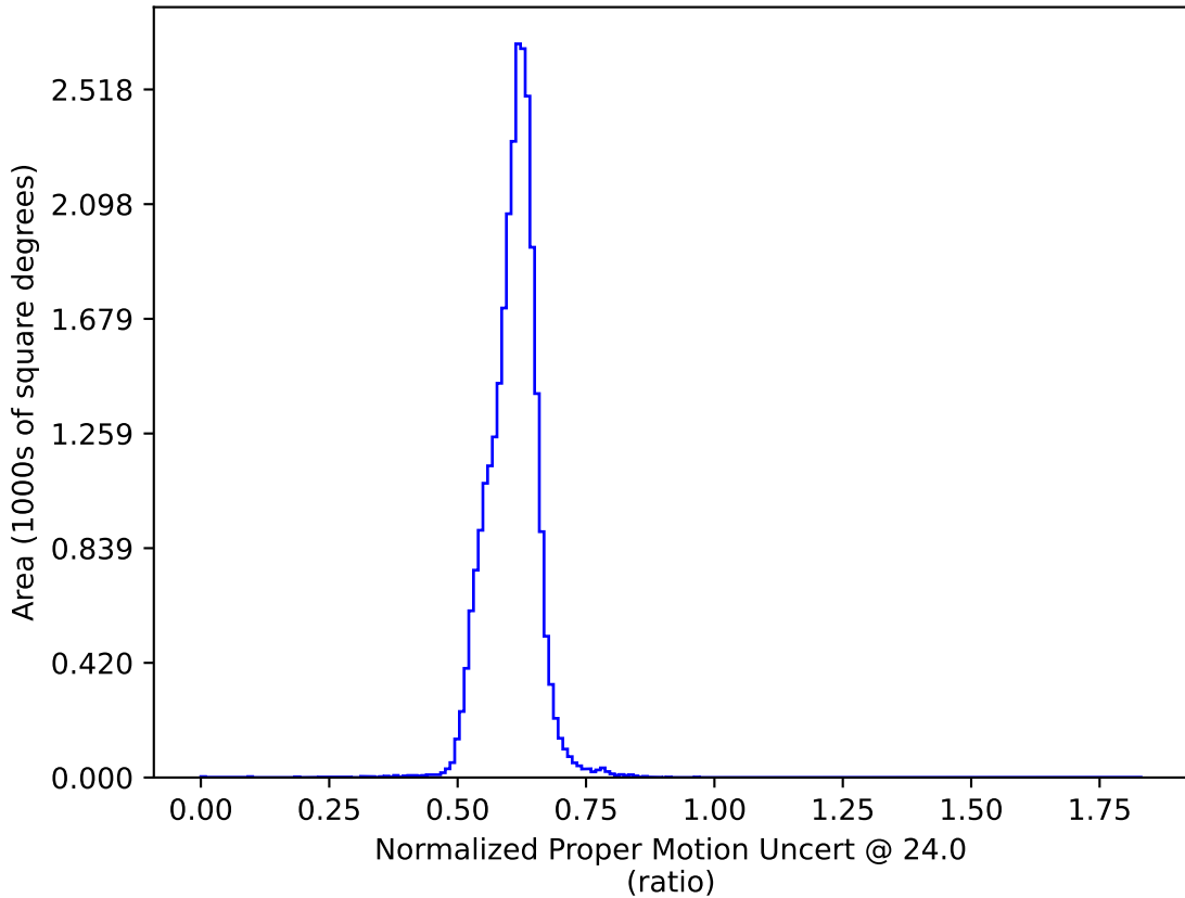
too_elab_r16_d2_giz_v3.4_10yrs : Normalized Proper Motion Uncert @ 24.0
