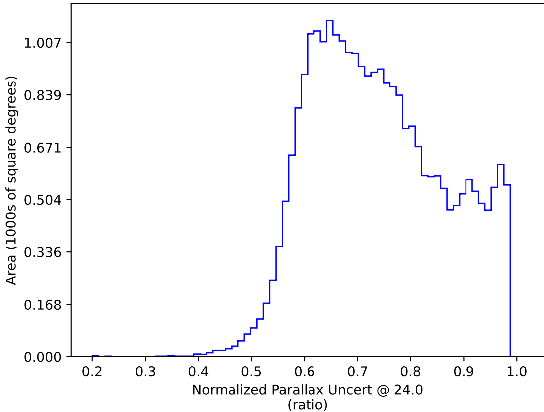
too_elab_r16_d2_giz_v3.4_10yrs : Normalized Parallax Uncert @ 24.0
