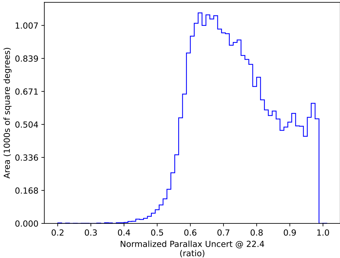
too_elab_r16_d2_giz_v3.4_10yrs : Normalized Parallax Uncert @ 22.4
