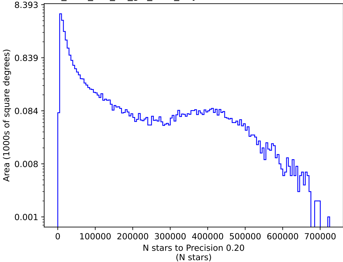
too_elab_r16_d2_giz_v3.4_10yrs i: N stars to Precision 0.20
