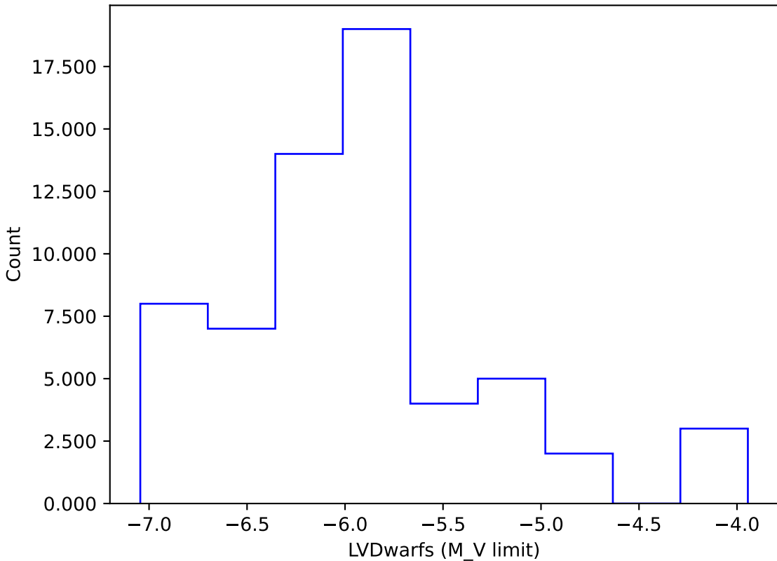
too_elab_r16_d2_giz_v3.4_10yrs gi: LVDwarfs
