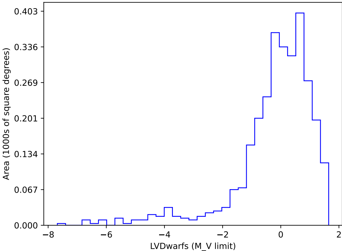
too_elab_r16_d2_giz_v3.4_10yrs gi SCP: LVDwarfs
