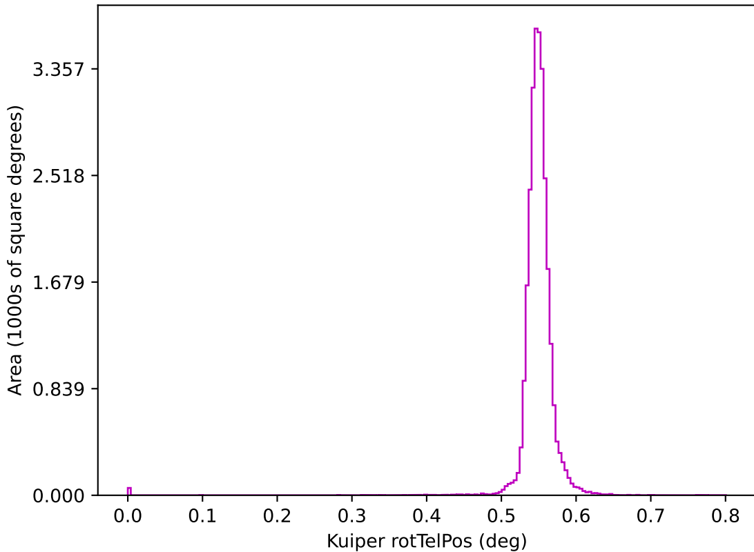
too_elab_r16_d2_giz_v3.4_10yrs z: Kuiper rotTelPos
