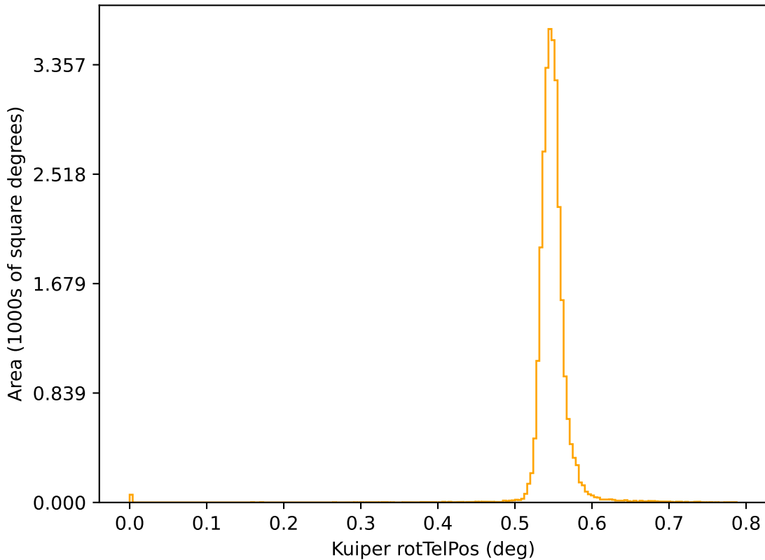
too_elab_r16_d2_giz_v3.4_10yrs r: Kuiper rotTelPos
