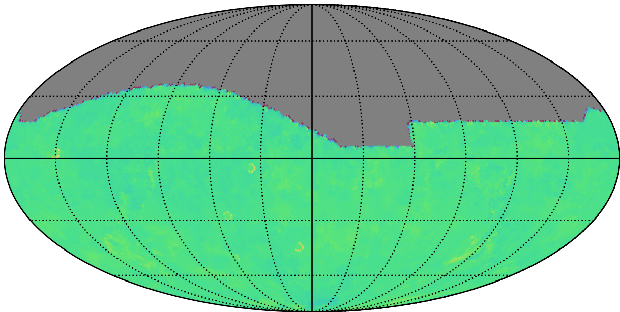
too_elab_r16_d2_giz_v3.4_10yrs g: Kuiper rotTelPos
