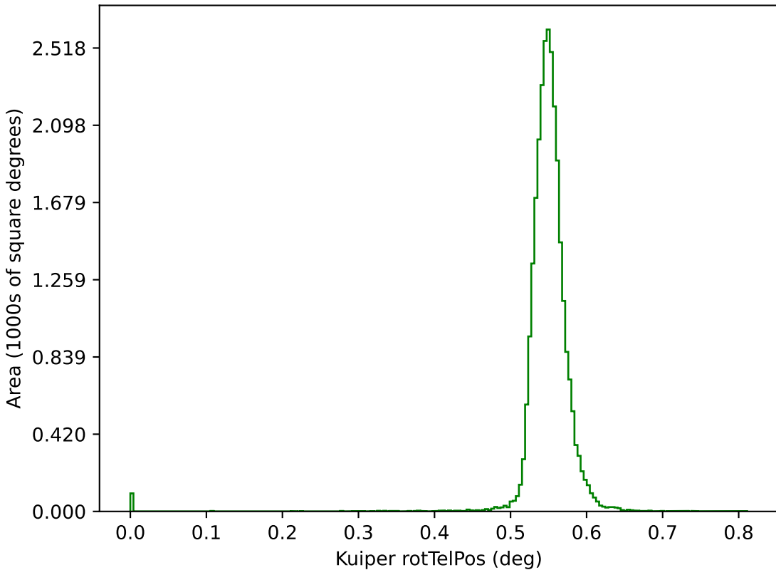
too_elab_r16_d2_giz_v3.4_10yrs g: Kuiper rotTelPos
