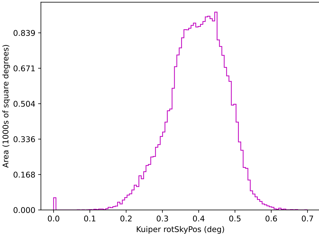
too_elab_r16_d2_giz_v3.4_10yrs z: Kuiper rotSkyPos
