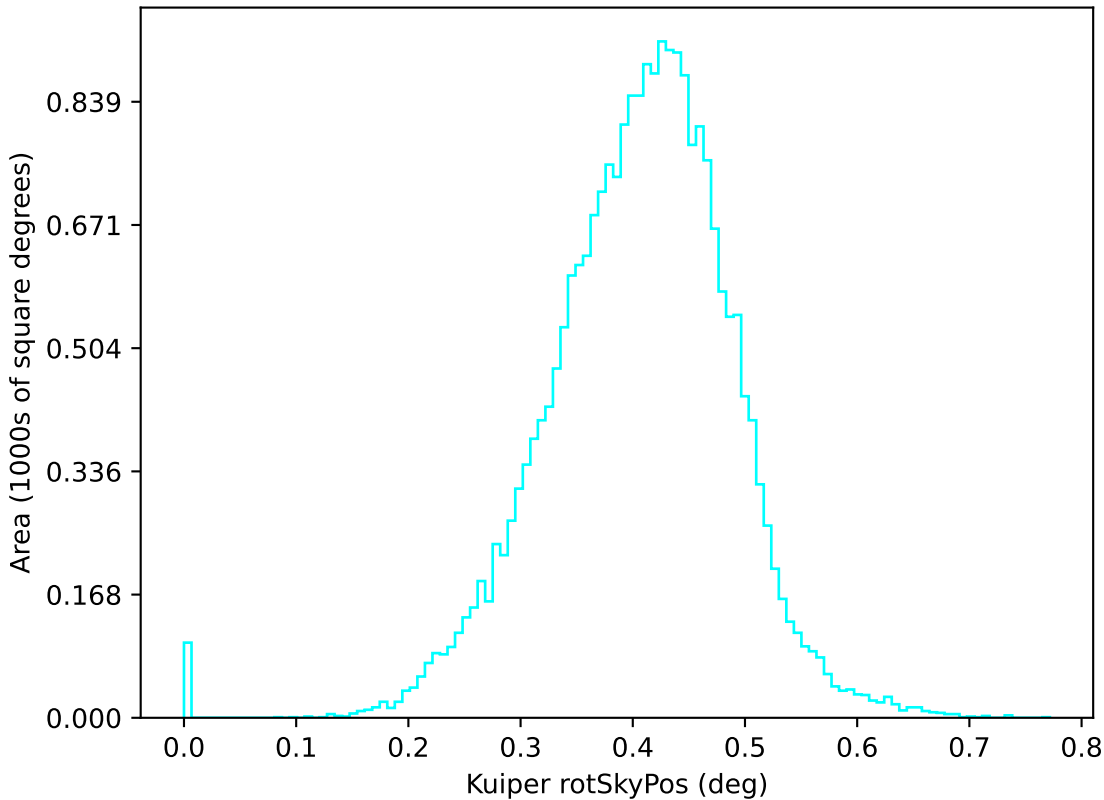
too_elab_r16_d2_giz_v3.4_10yrs u: Kuiper rotSkyPos
