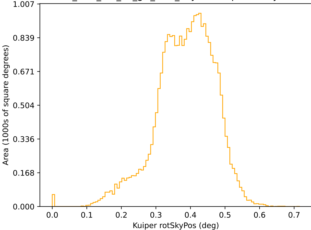
too_elab_r16_d2_giz_v3.4_10yrs r: Kuiper rotSkyPos
