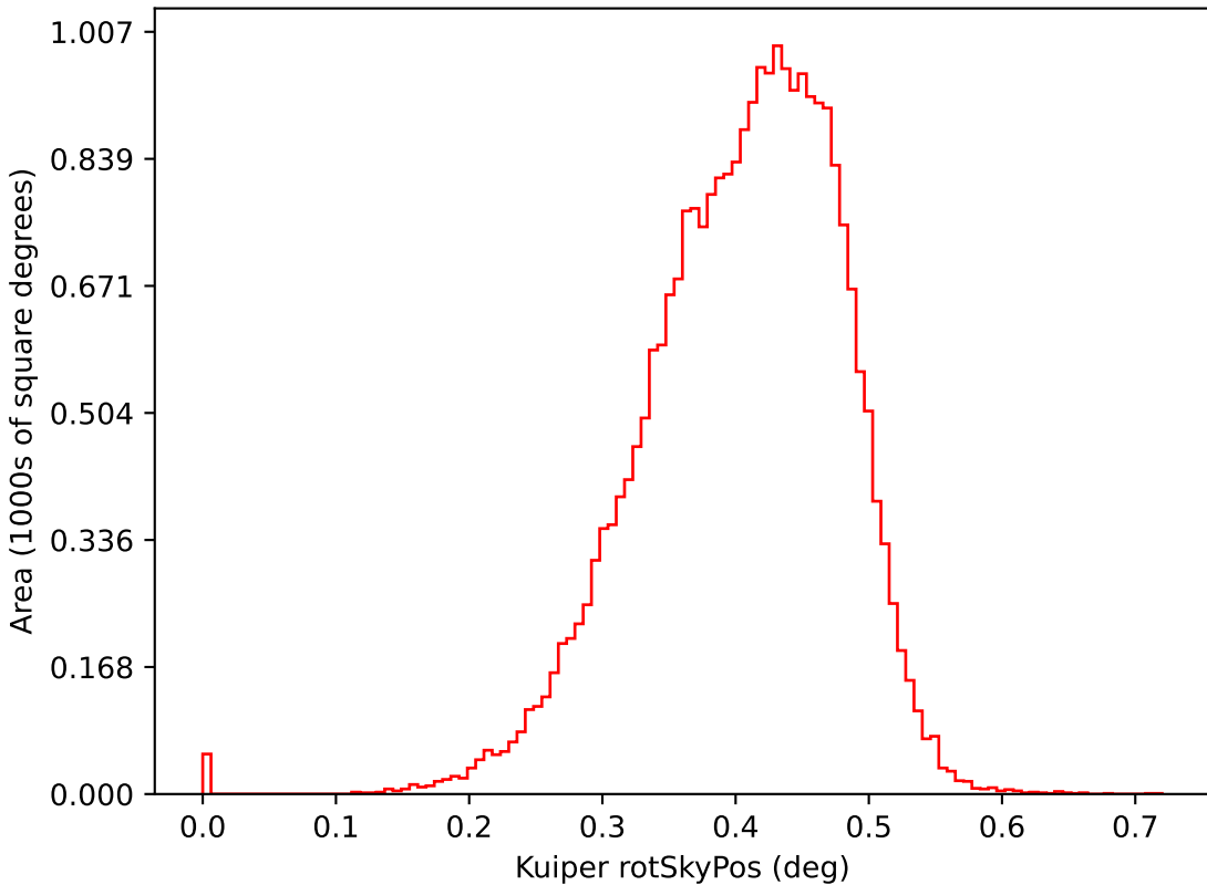
too_elab_r16_d2_giz_v3.4_10yrs i: Kuiper rotSkyPos
