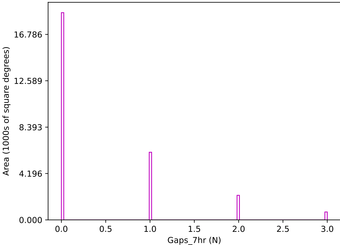
too_elab_r16_d2_giz_v3.4_10yrs z band: Gaps_7hr
