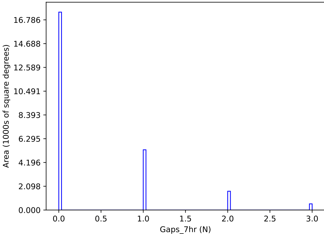
too_elab_r16_d2_giz_v3.4_10yrs y band: Gaps_7hr
