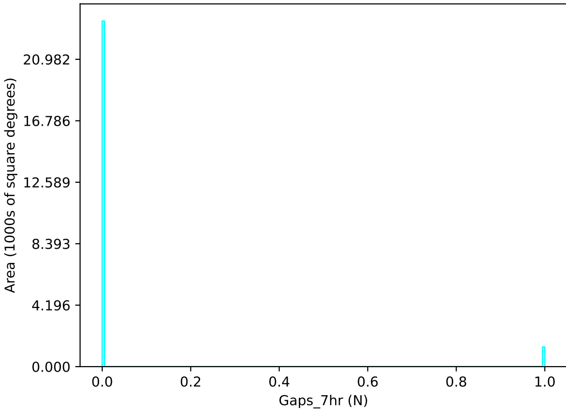
too_elab_r16_d2_giz_v3.4_10yrs u band: Gaps_7hr
