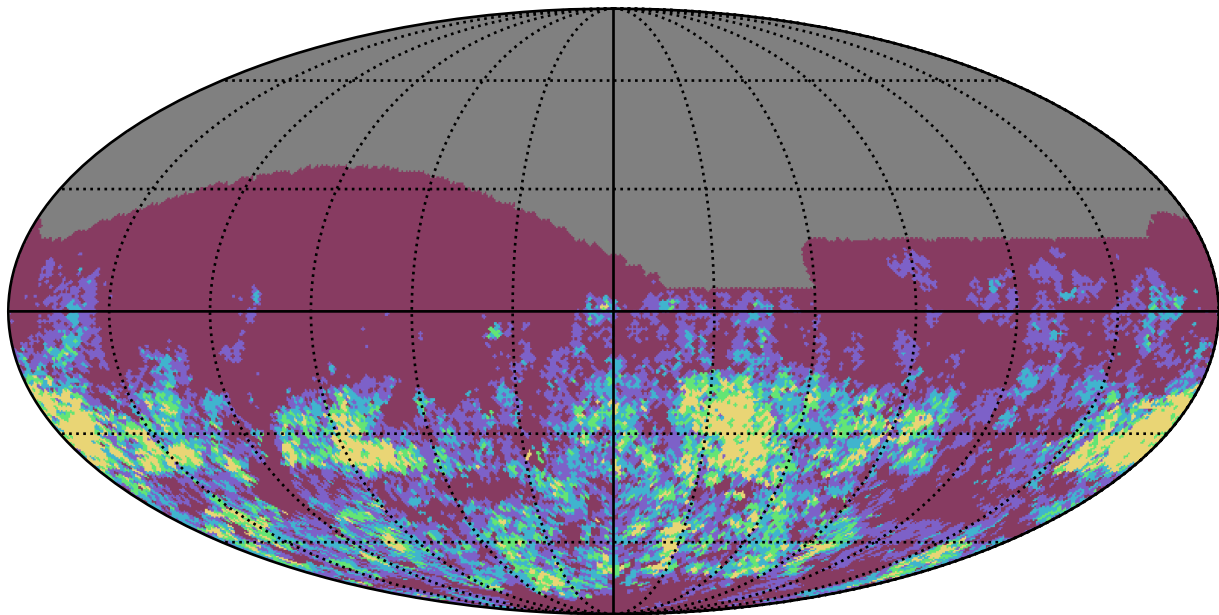
too_elab_r16_d2_giz_v3.4_10yrs r band: Gaps_7hr
