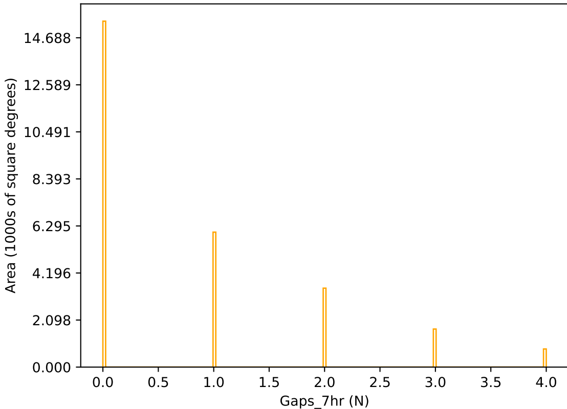
too_elab_r16_d2_giz_v3.4_10yrs r band: Gaps_7hr
