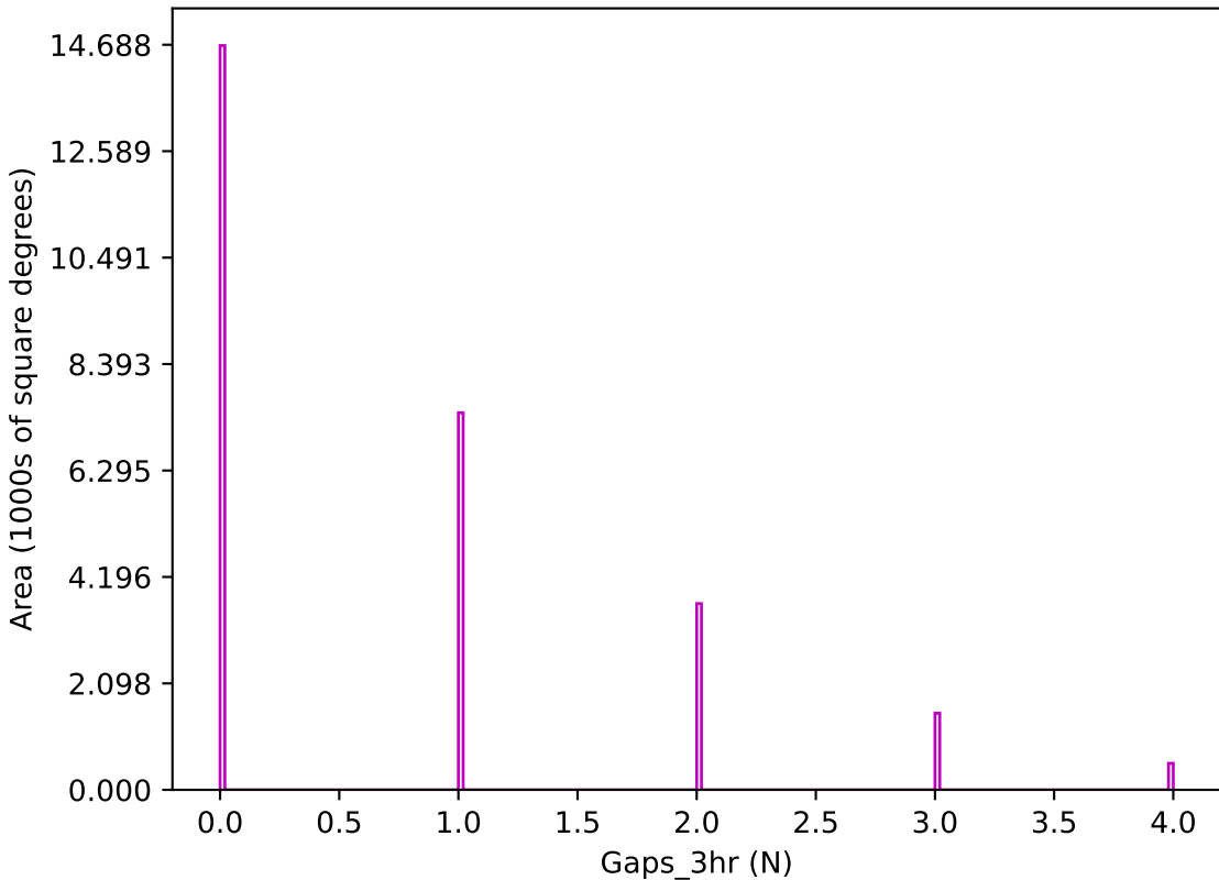
too_elab_r16_d2_giz_v3.4_10yrs z band: Gaps_3hr
