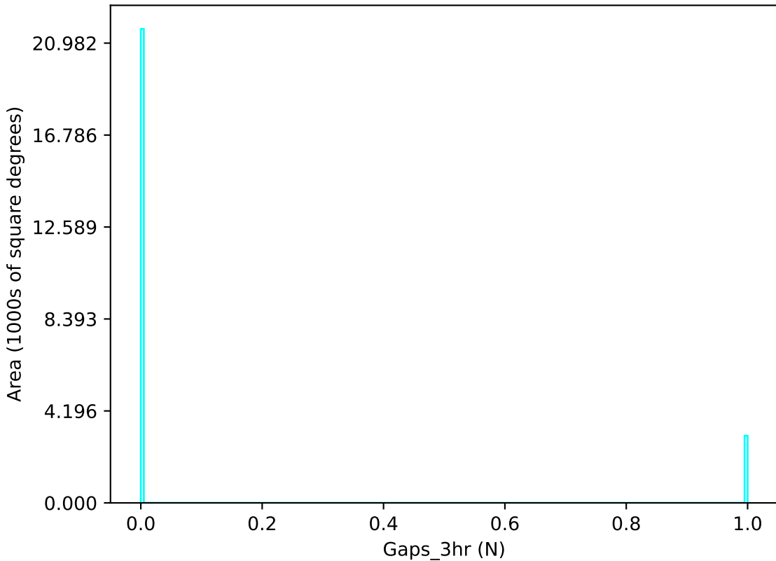
too_elab_r16_d2_giz_v3.4_10yrs u band: Gaps_3hr
