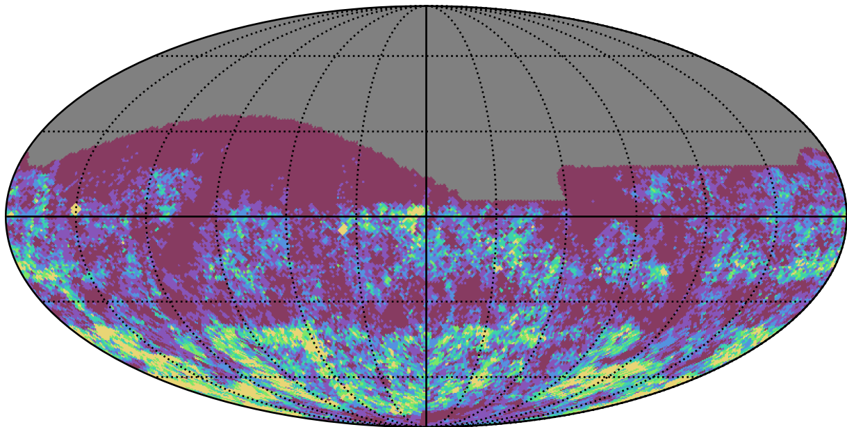
too_elab_r16_d2_giz_v3.4_10yrs r band: Gaps_3hr
