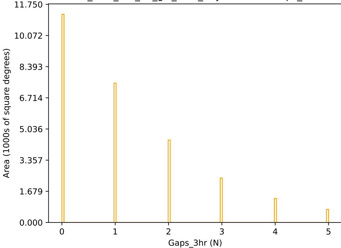
too_elab_r16_d2_giz_v3.4_10yrs r band: Gaps_3hr
