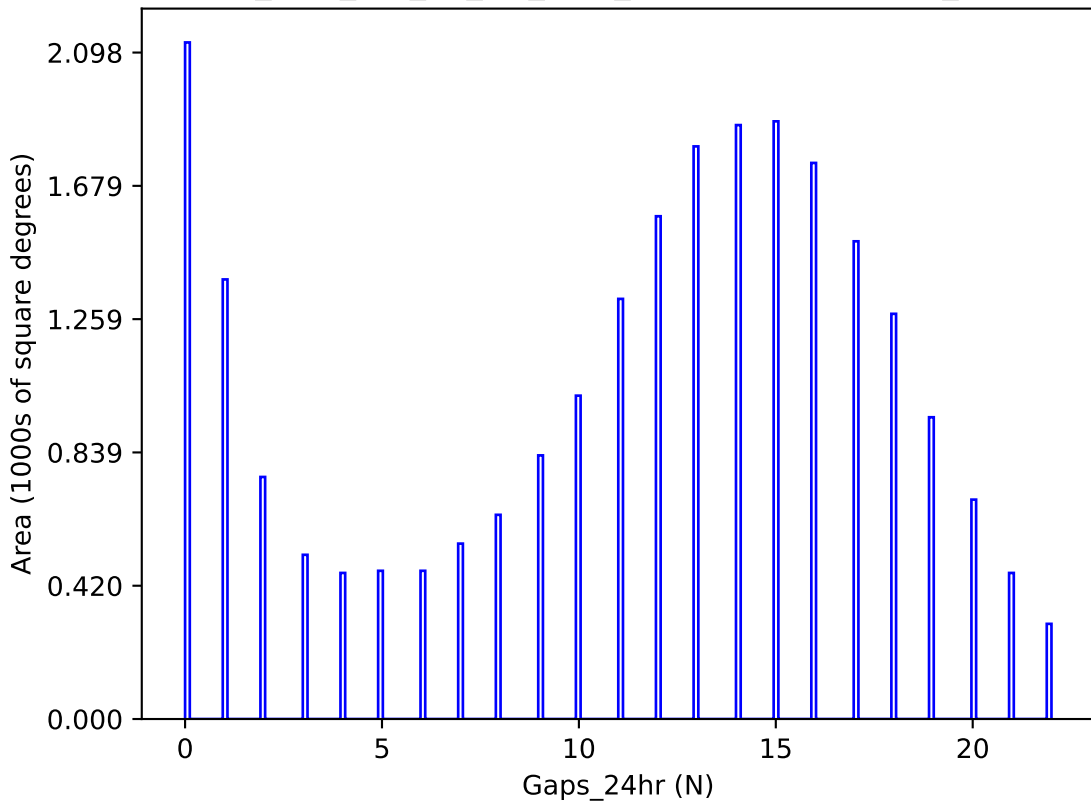
too_elab_r16_d2_giz_v3.4_10yrs y band: Gaps_24hr
