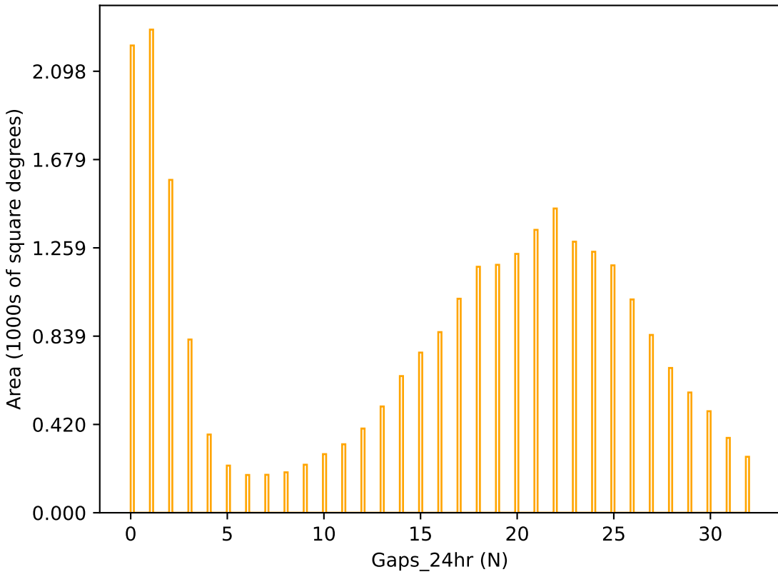
too_elab_r16_d2_giz_v3.4_10yrs r band: Gaps_24hr
