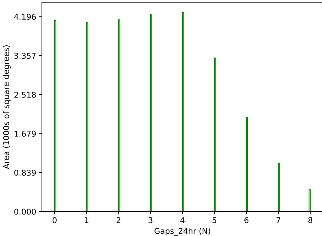
too_elab_r16_d2_giz_v3.4_10yrs g band: Gaps_24hr
