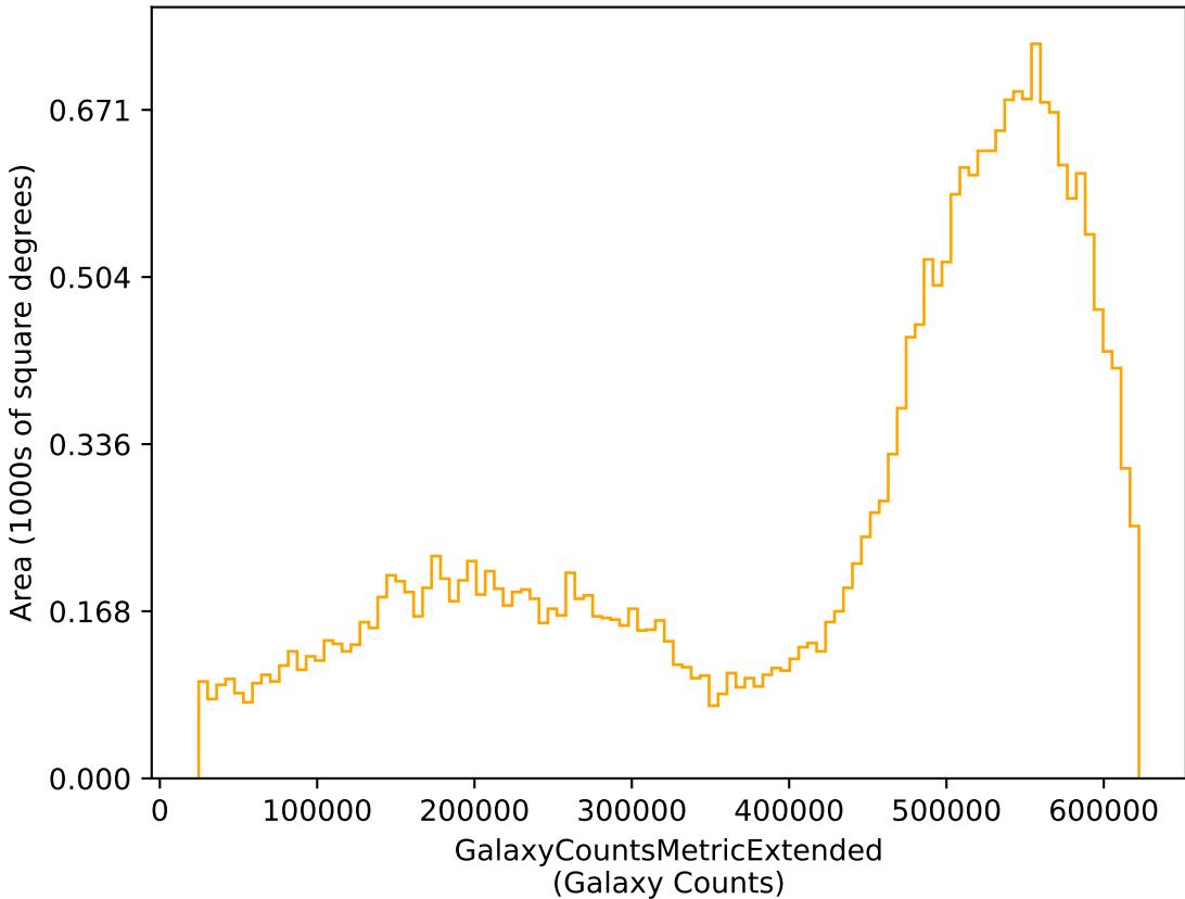
too_elab_r16_d2_giz_v3.4_10yrs r: GalaxyCountsMetricExtended
