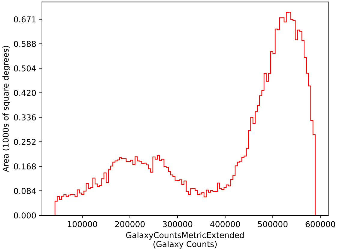
too_elab_r16_d2_giz_v3.4_10yrs i: GalaxyCountsMetricExtended
