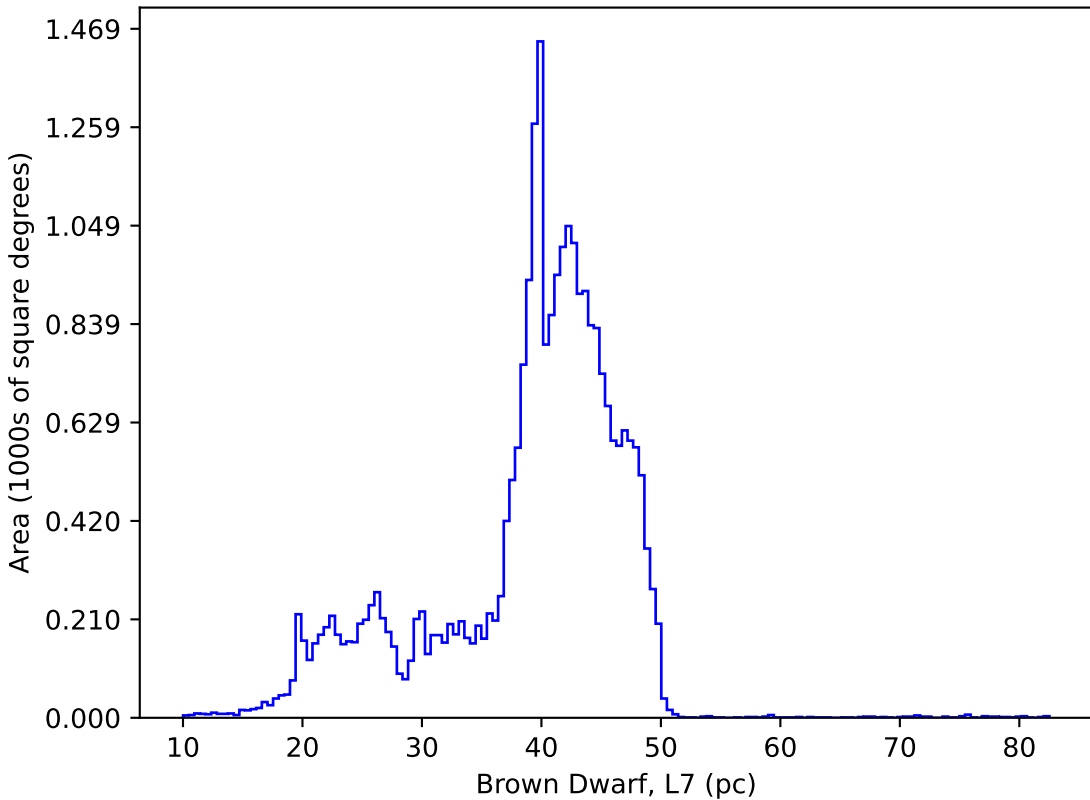
too_elab_r16_d2_giz_v3.4_10yrs : Brown Dwarf, L7
