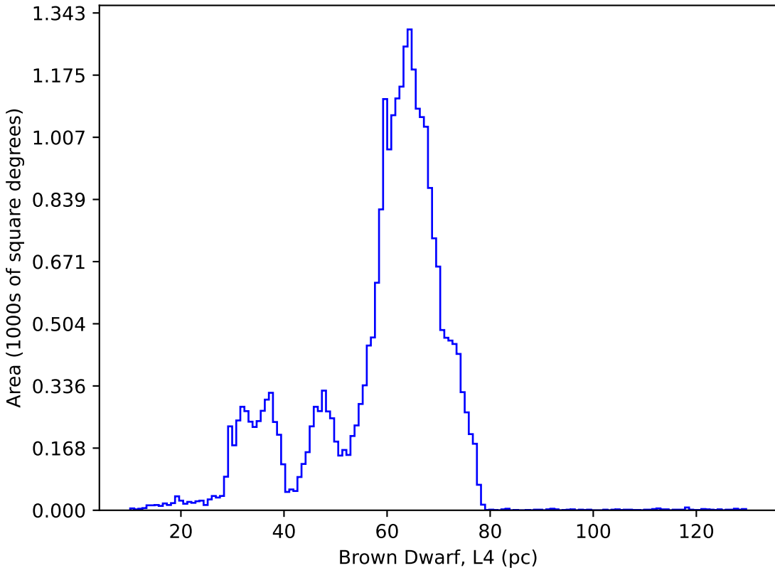
too_elab_r16_d2_giz_v3.4_10yrs : Brown Dwarf, L4
