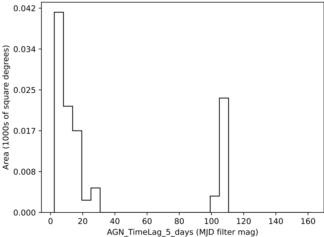
too_elab_r16_d2_giz_v3.4_10yrs all bands: AGN_TimeLag_5_days
