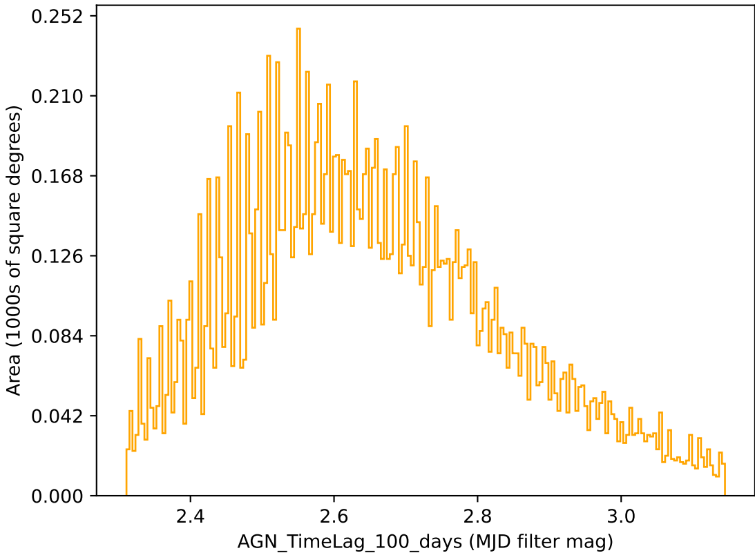
too_elab_r16_d2_giz_v3.4_10yrs r band: AGN_TimeLag_100_days
