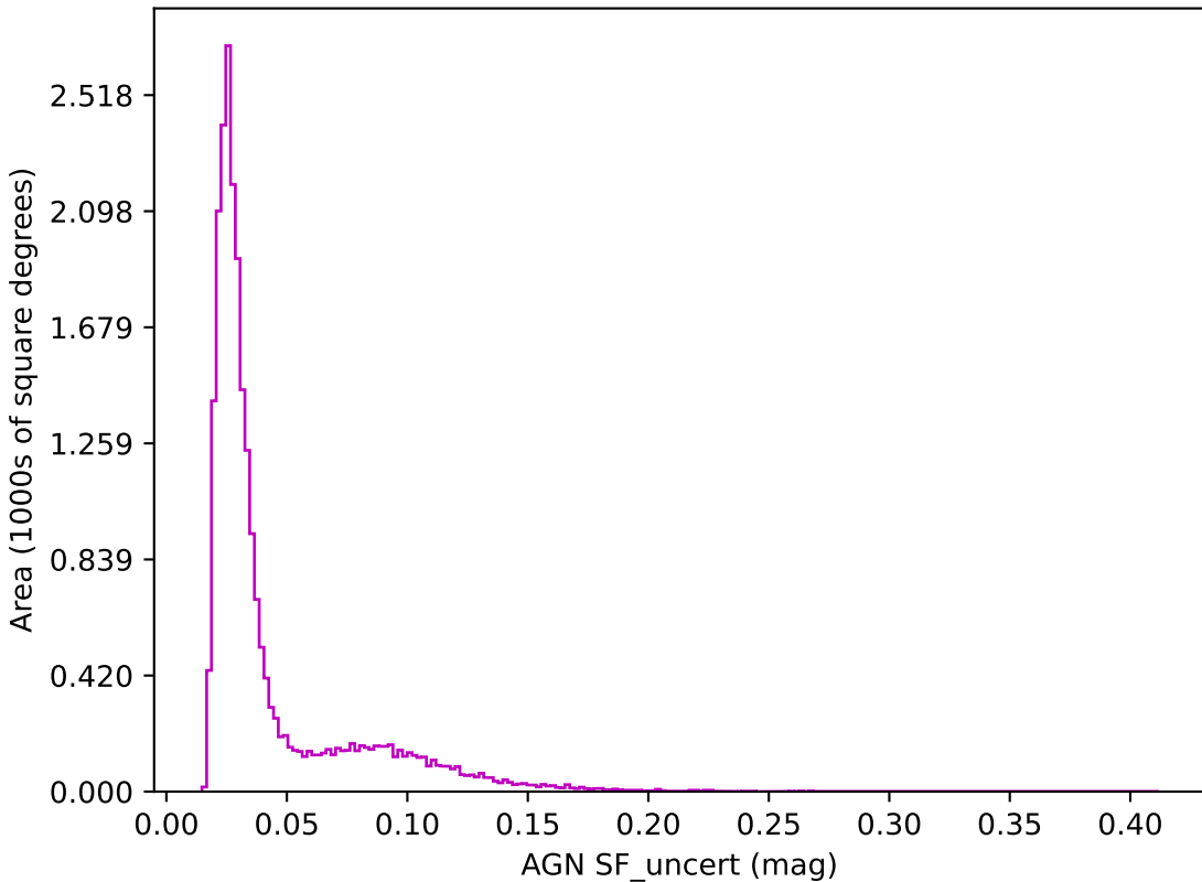
too_elab_r16_d2_giz_v3.4_10yrs z band: AGN SF_uncert
