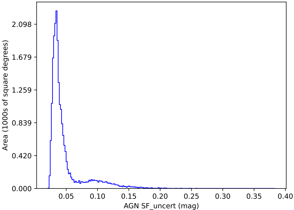
too_elab_r16_d2_giz_v3.4_10yrs y band: AGN SF_uncert
