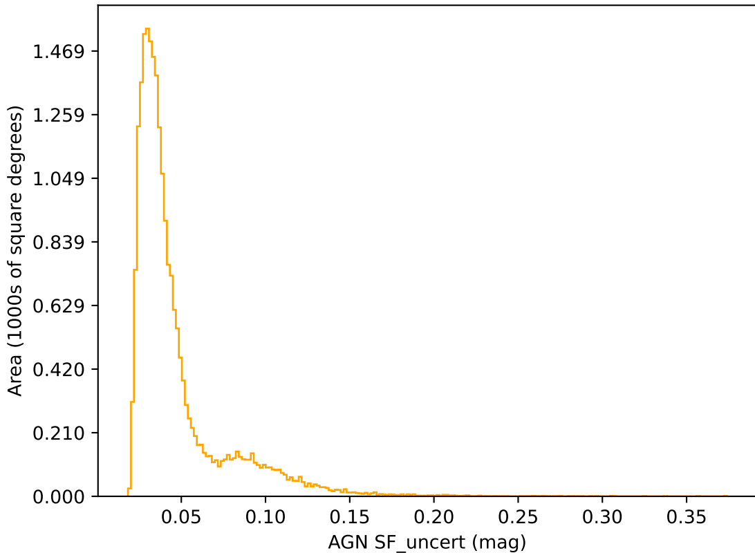
too_elab_r16_d2_giz_v3.4_10yrs r band: AGN SF_uncert
