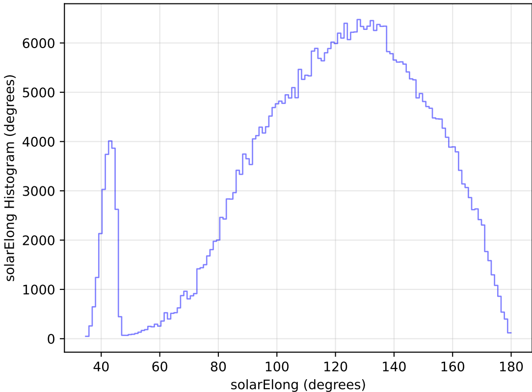
too_elab_r16_d2_giz_v3.4_10yrs WFD z band: solarElong Histogram
