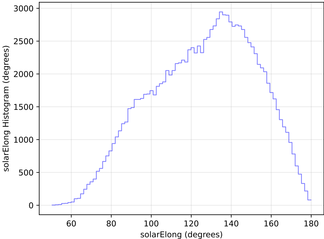
too_elab_r16_d2_giz_v3.4_10yrs WFD u band: solarElong Histogram
